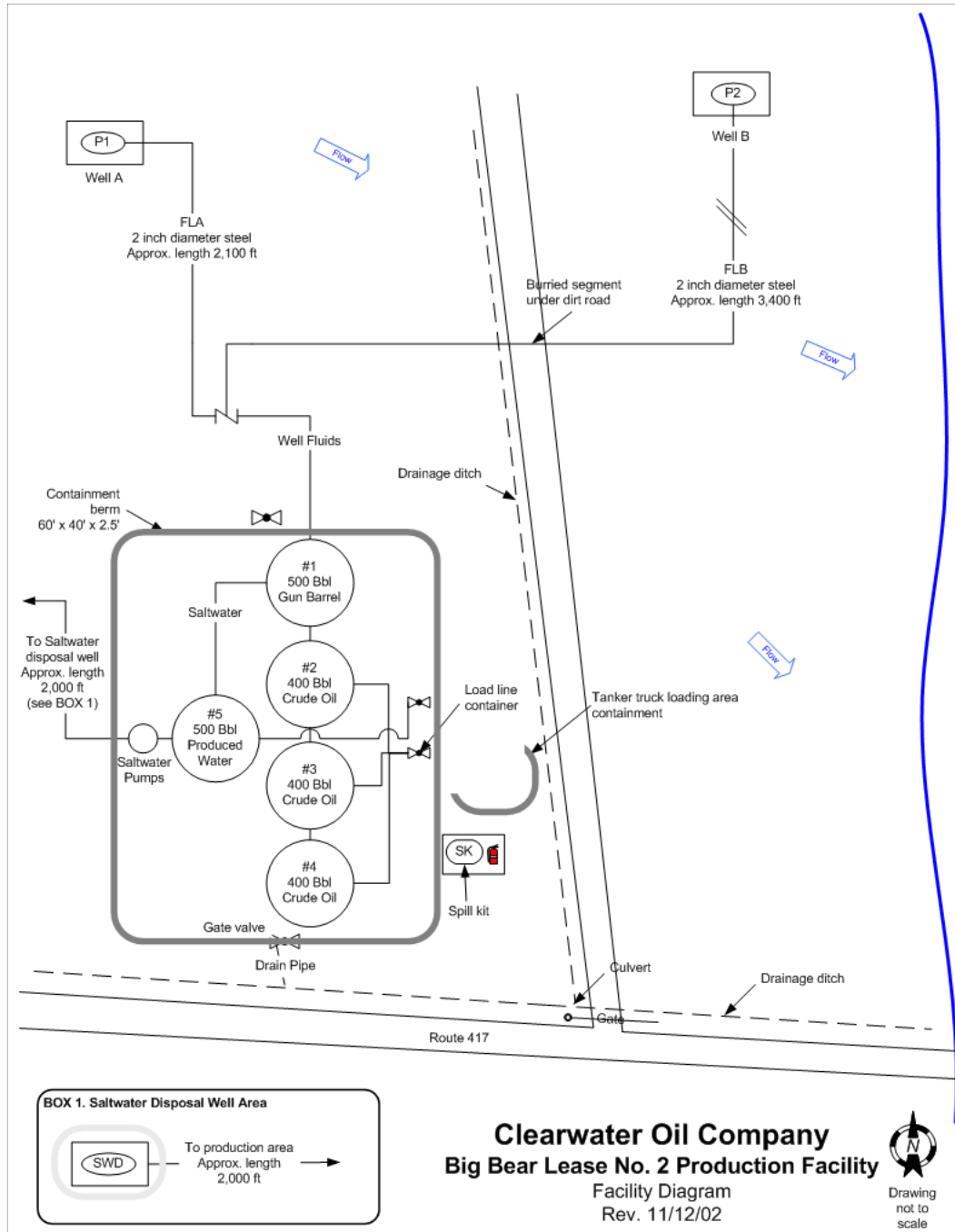
Figure C-2: Facility Diagram.
