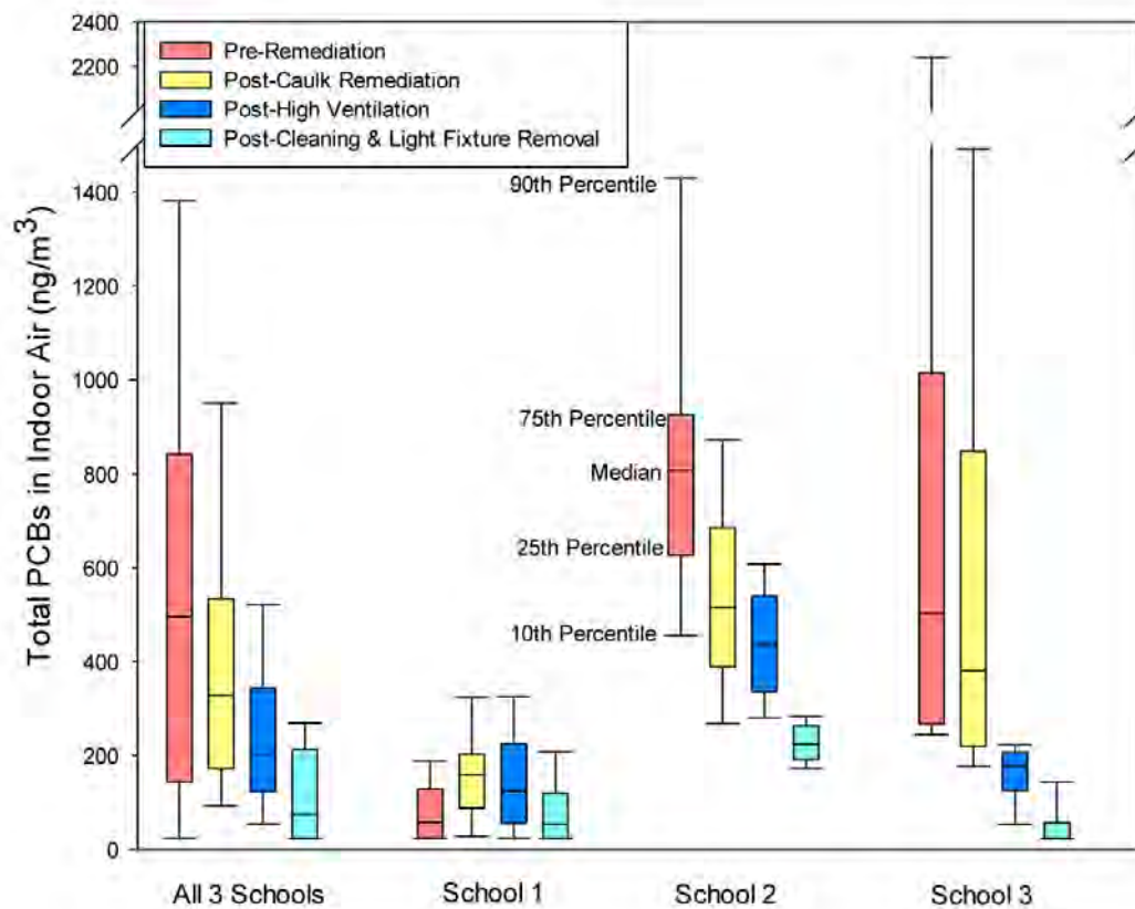
Figure 4-11. Pre- and post-remediation indoor air total PCB concentrations across three schools with several different remedial activities.
