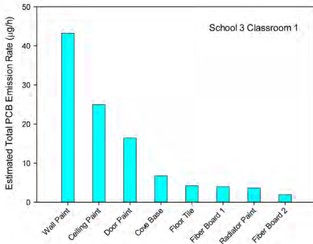
Figure 4-4. Screening-level estimates of total PCB emission rates from materials in a classroom in School 3
