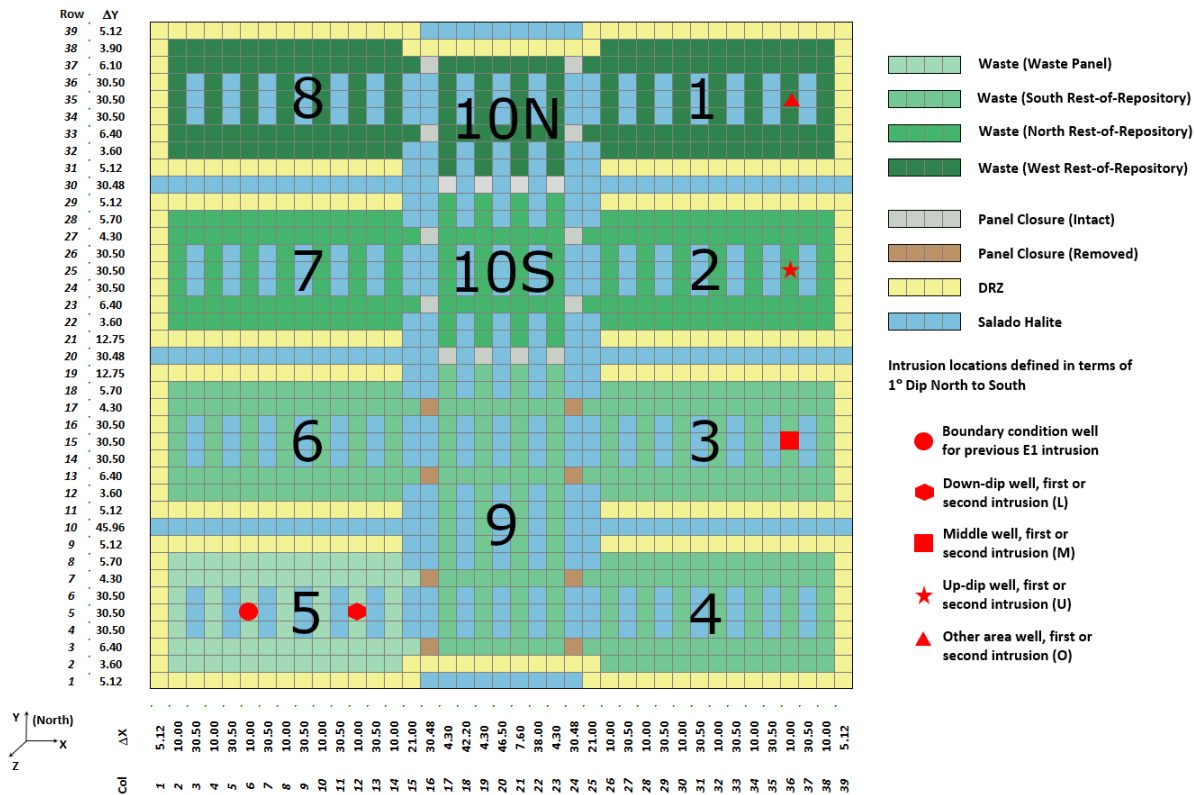
Figure 2-4: BRAGFLO Grid used in CRA19_12P DBR Calculations with Modeled Area Descriptions (Δx and Δy Dimensions in Meters)
