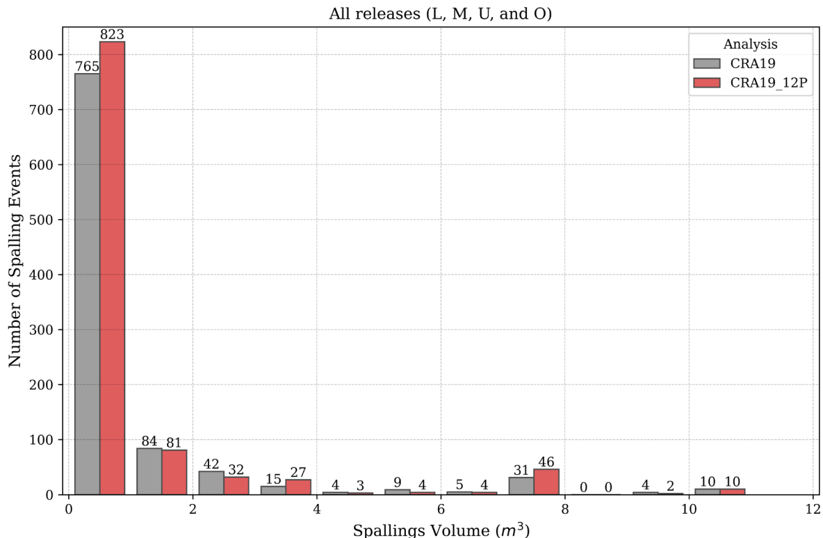
Figure 6-1: Number of Non-zero Spalling Events by Volume (All Intrusion Locations)
