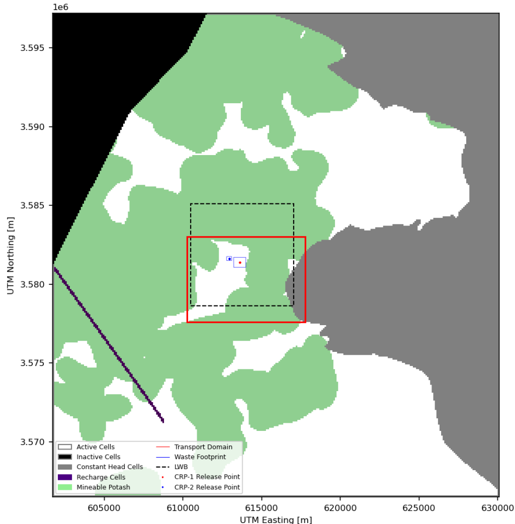
Figure 9-1: Culebra Flow and Transport Model Domain
