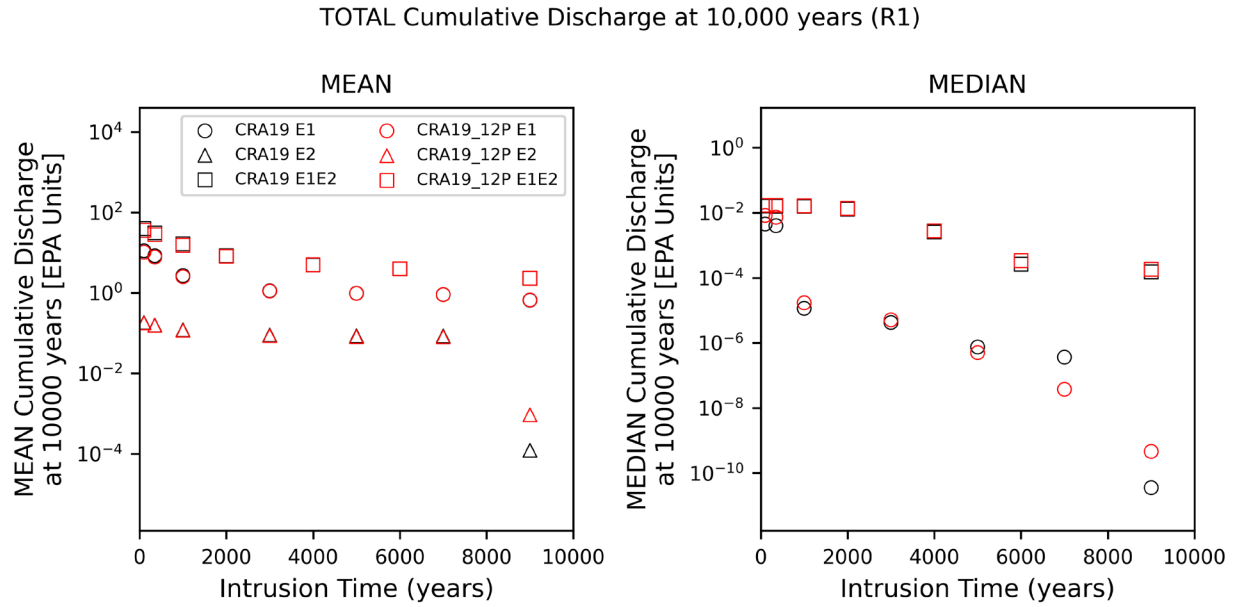
Figure 8-4: Mean and Median Cumulative Discharges of Total Radionuclides to the Culebra at 10,000 Years.
