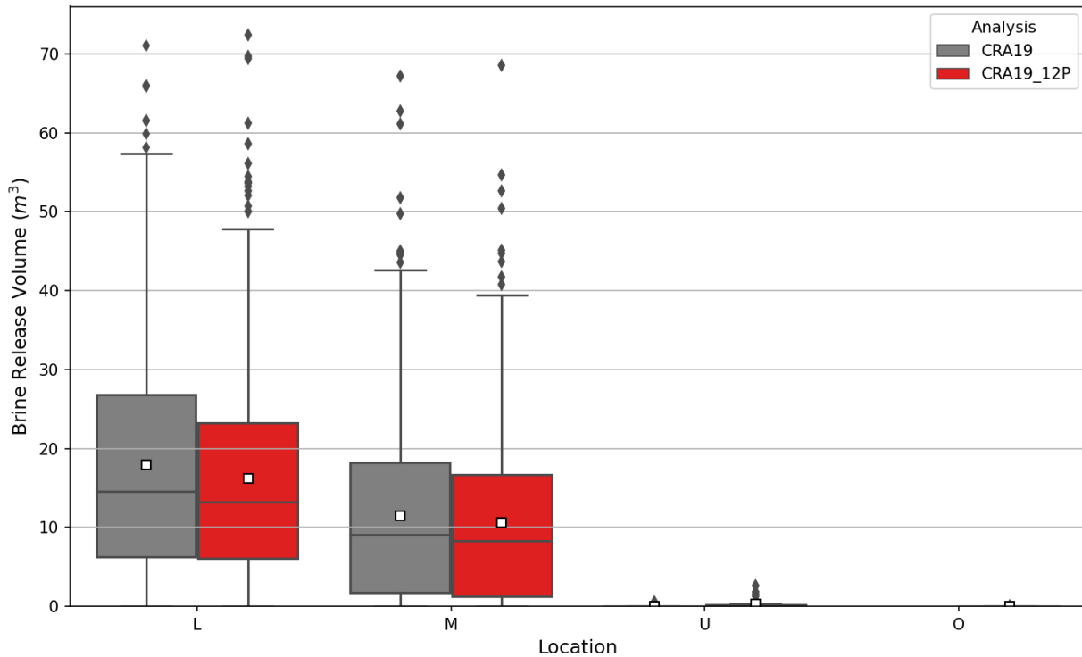
Figure 5-5: Release Volumes by Location; All Non-zero Releases
