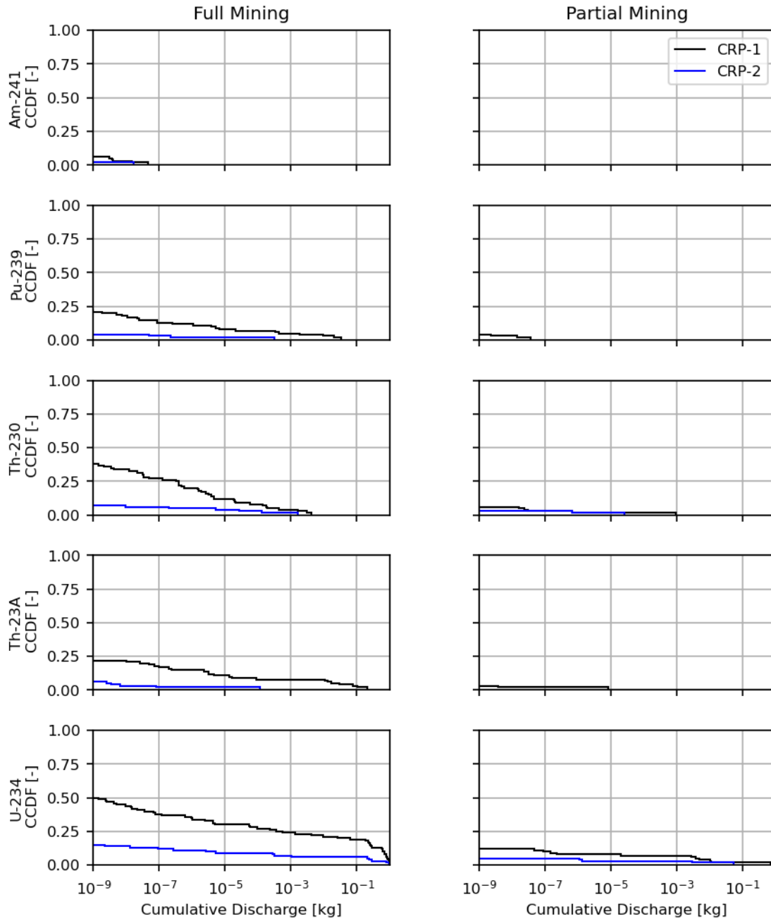
Figure 9-5: Cumulative Mass Discharge to the LWB by t=10,000 yrs
